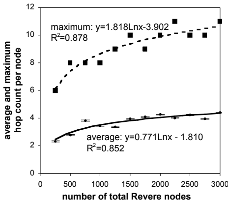
Fig. 9. Average and maximum hop count of security update dissemination (confidence level for average hop count: 99.9%)
