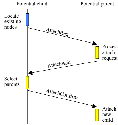
Fig. 1. Three-way-handshake protocol
