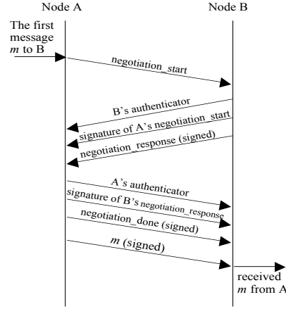
Fig. 5. Authentication scheme negotiation
