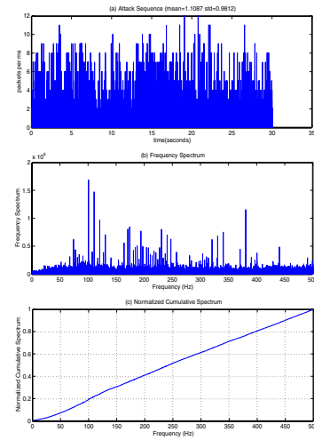
Figure 7. Frequency spectrum of a centralized attack
