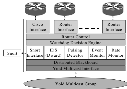
Figure 3. Watchdog architecture
